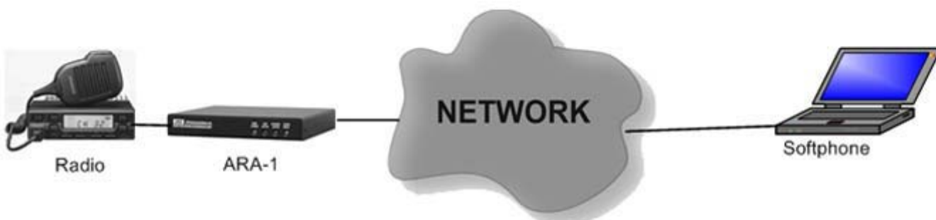
SIP Example use over Internet
