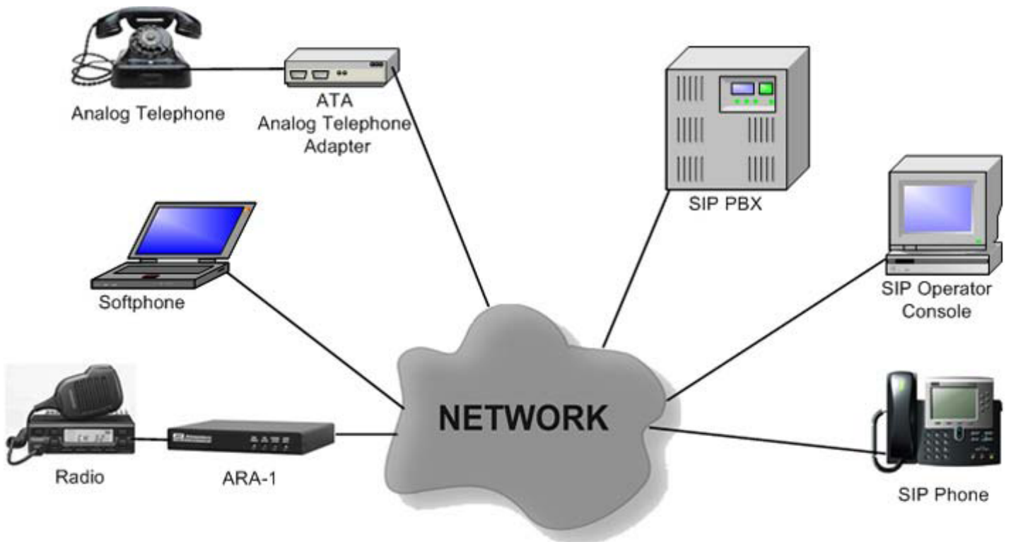
Operation with SIP PBX Network
