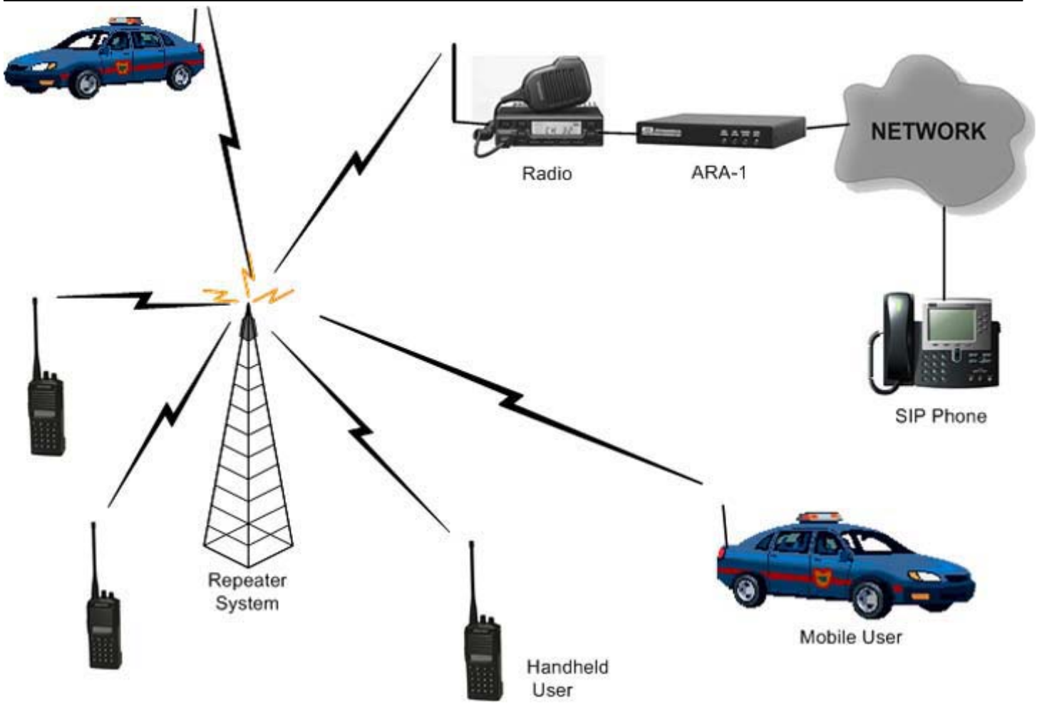
SIP with Repeater System
